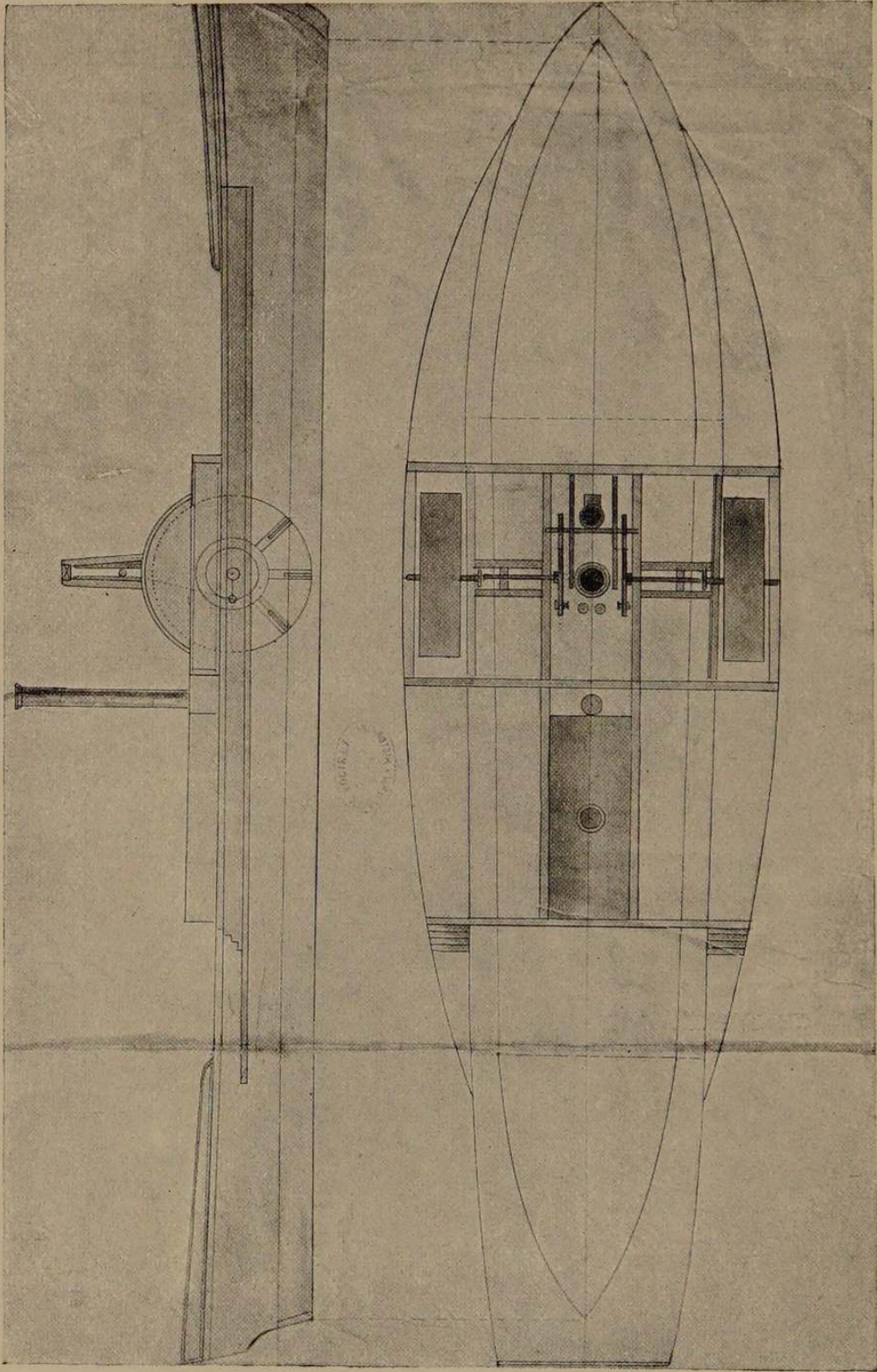
C. FULTON'S PLAN OF A LATER STEAMBOAT, SHOWING APPLICATION OF THE SQUARE SIDE-CONNECTING-ROD ENGINE, THE INVENTION OF WHICH HE ASCRIBES TO JOHN STEVENS
