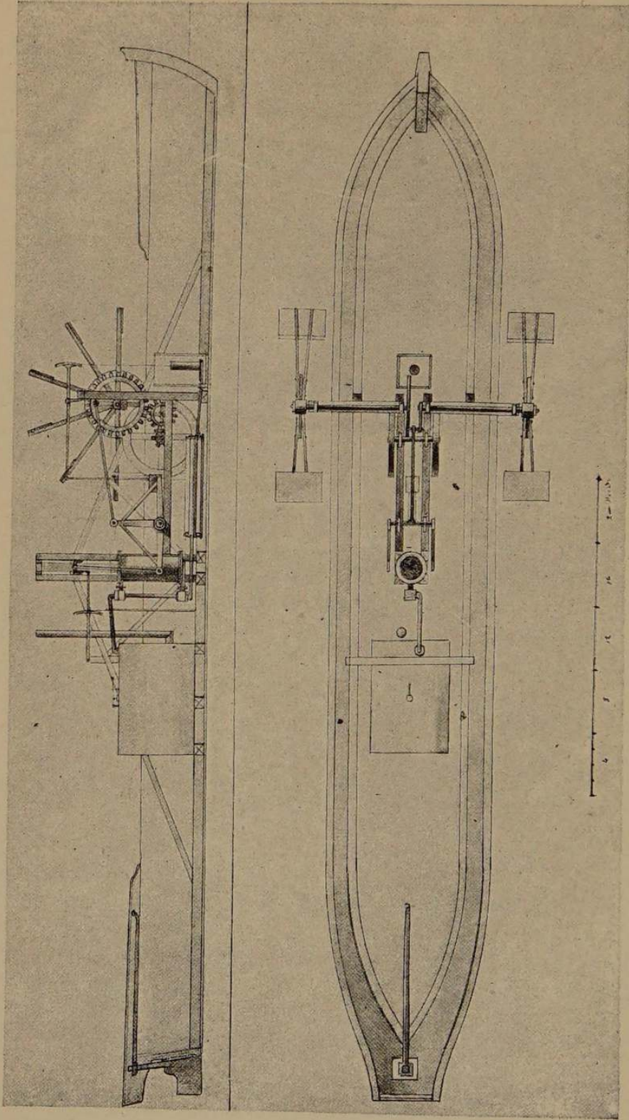
FULTON'S DRAWING FOR A STEAMBOAT SUBMITTED TO THE COMMISSION APPOINTED BY NAPOLEON IN 1803 From the original drawing in the Conservatoire Des Arts et Métiers, Paris. From a photograph lent by "Cassier's Magazine"
