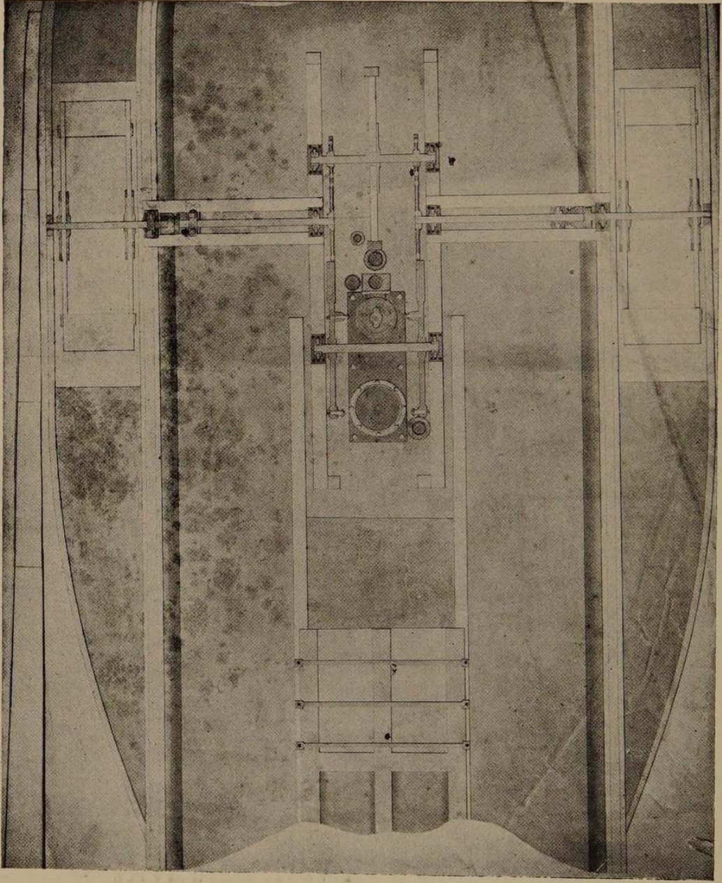
A. FULTON'S PLAN OF THE MACHINERY OF THE NORTH RIVER (THE REMODELED CLERMONT)
