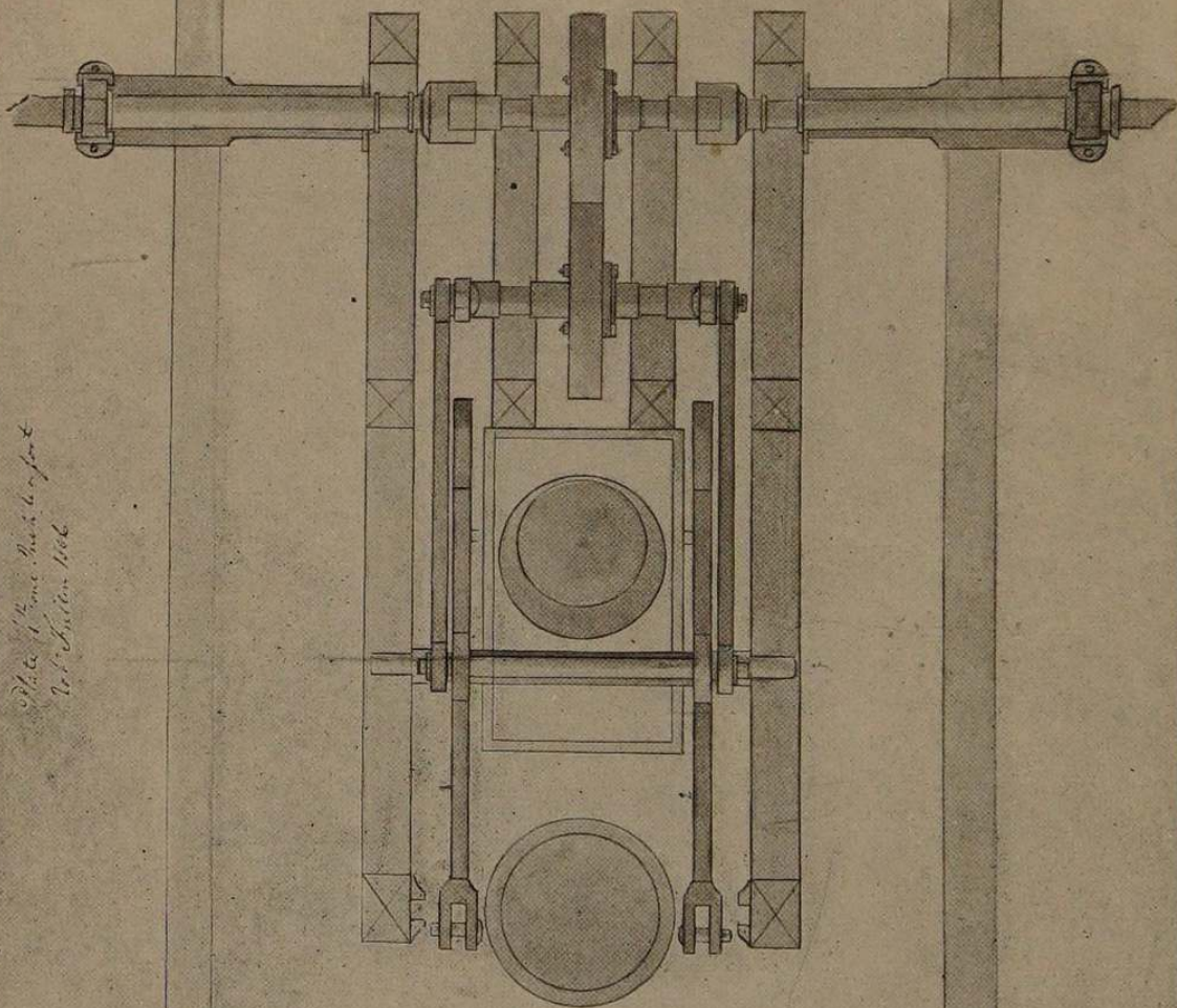
"PLATE 4." FULTON'S PRELIMINARY STUDY FOR THE CLERMONT'S ENGINE From the original in the New Jersey Historical Society. Now first published
